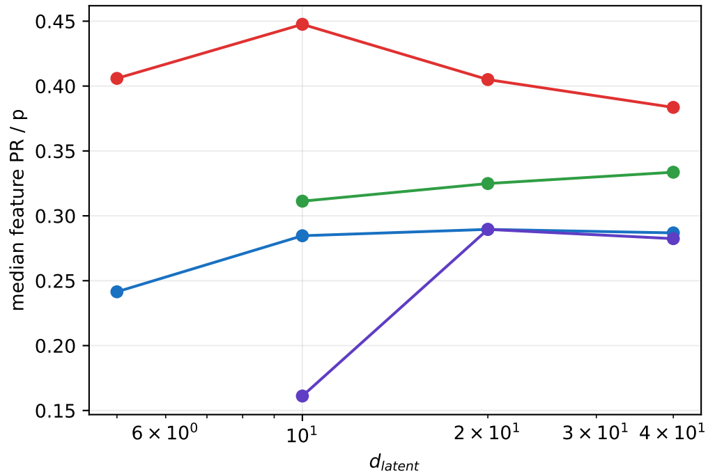
Feature-eigenvector participation ratio: p64
